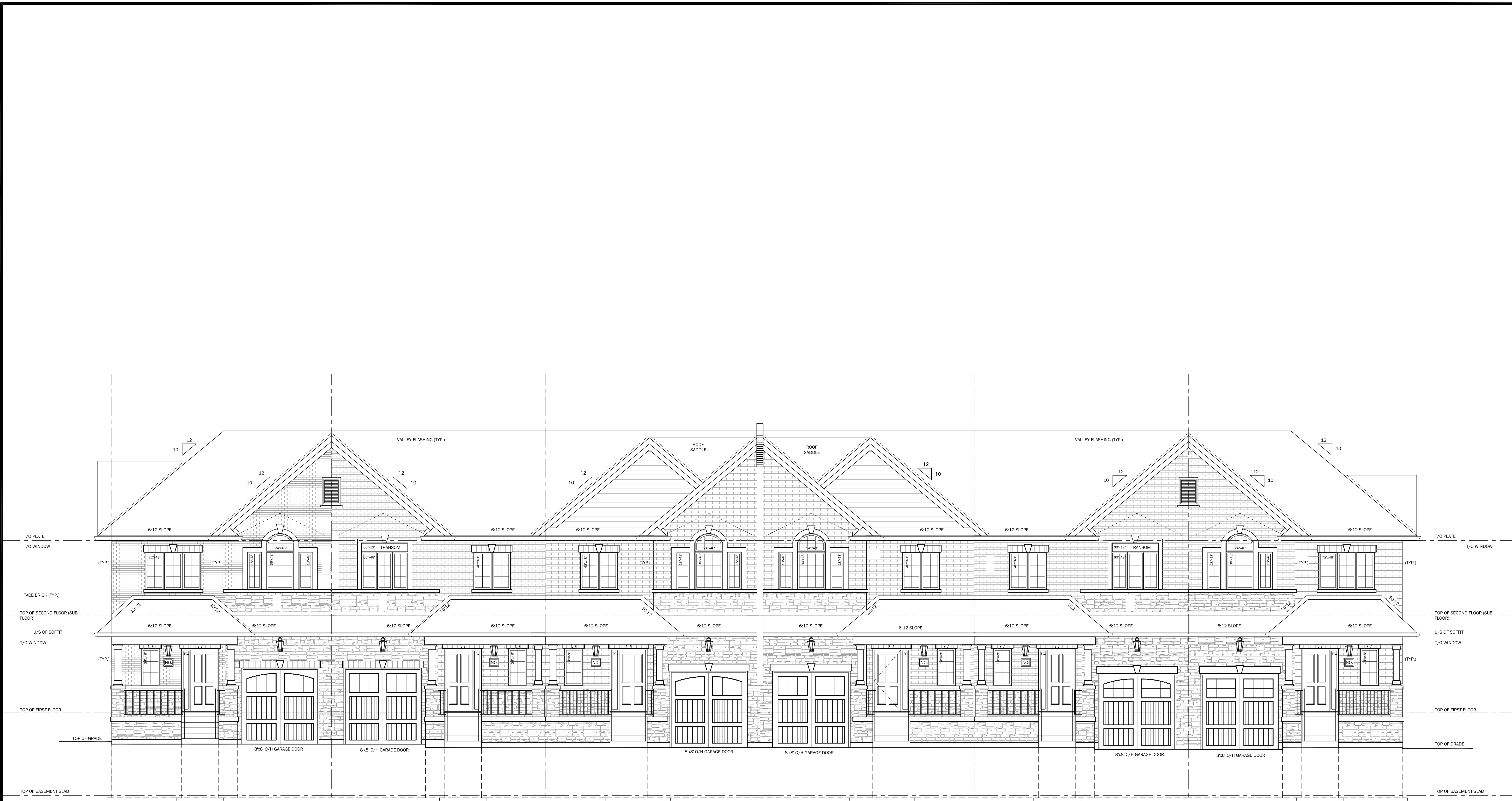
Front Elevation 'A'/Block Plan Scale 3/16" = 1'-0"
